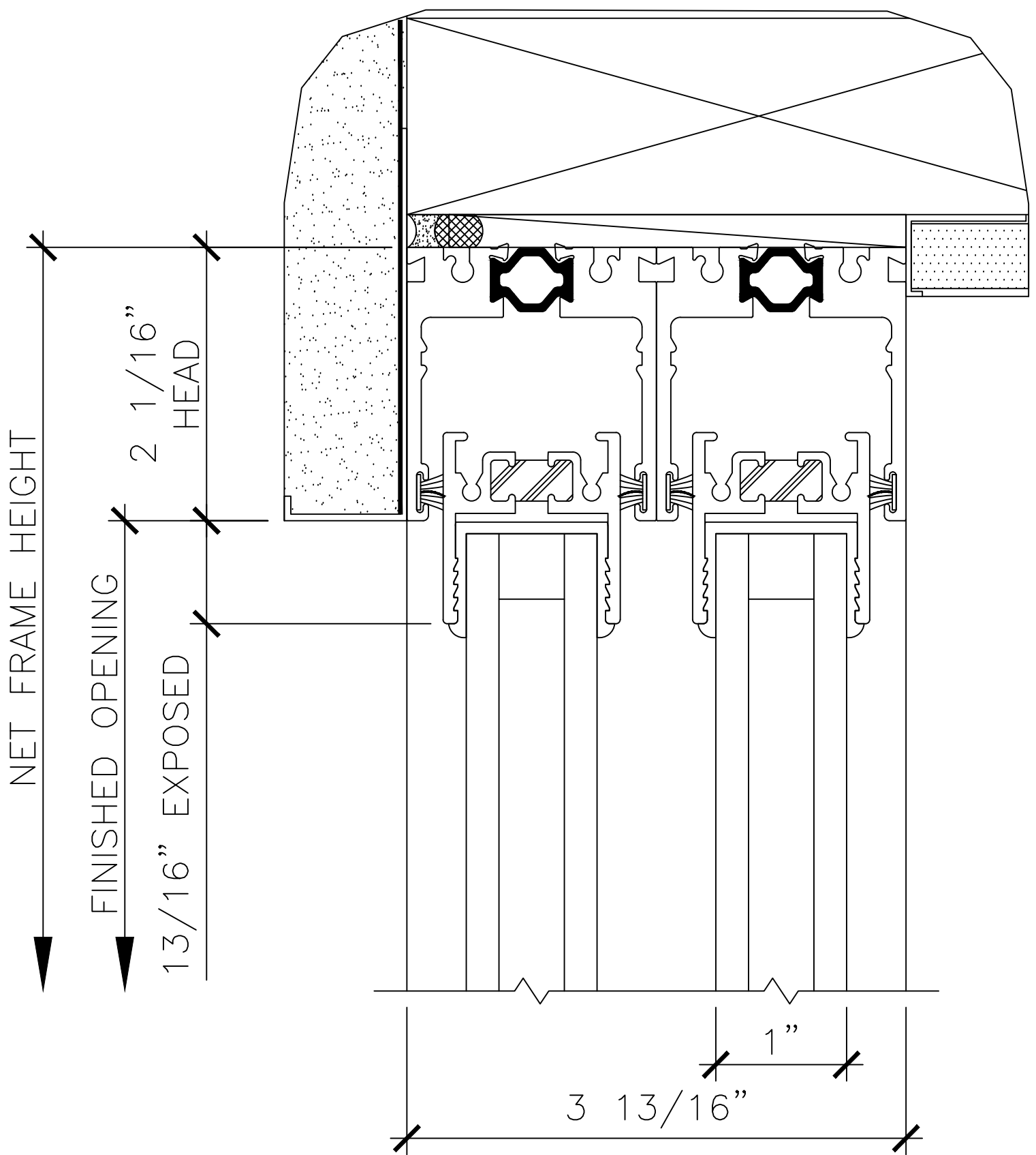
SERIES 3070-T HEAD
